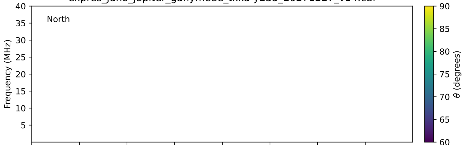
expres_juno_jupiter_ganymede_txka-y235_20271227_v14.cdf
