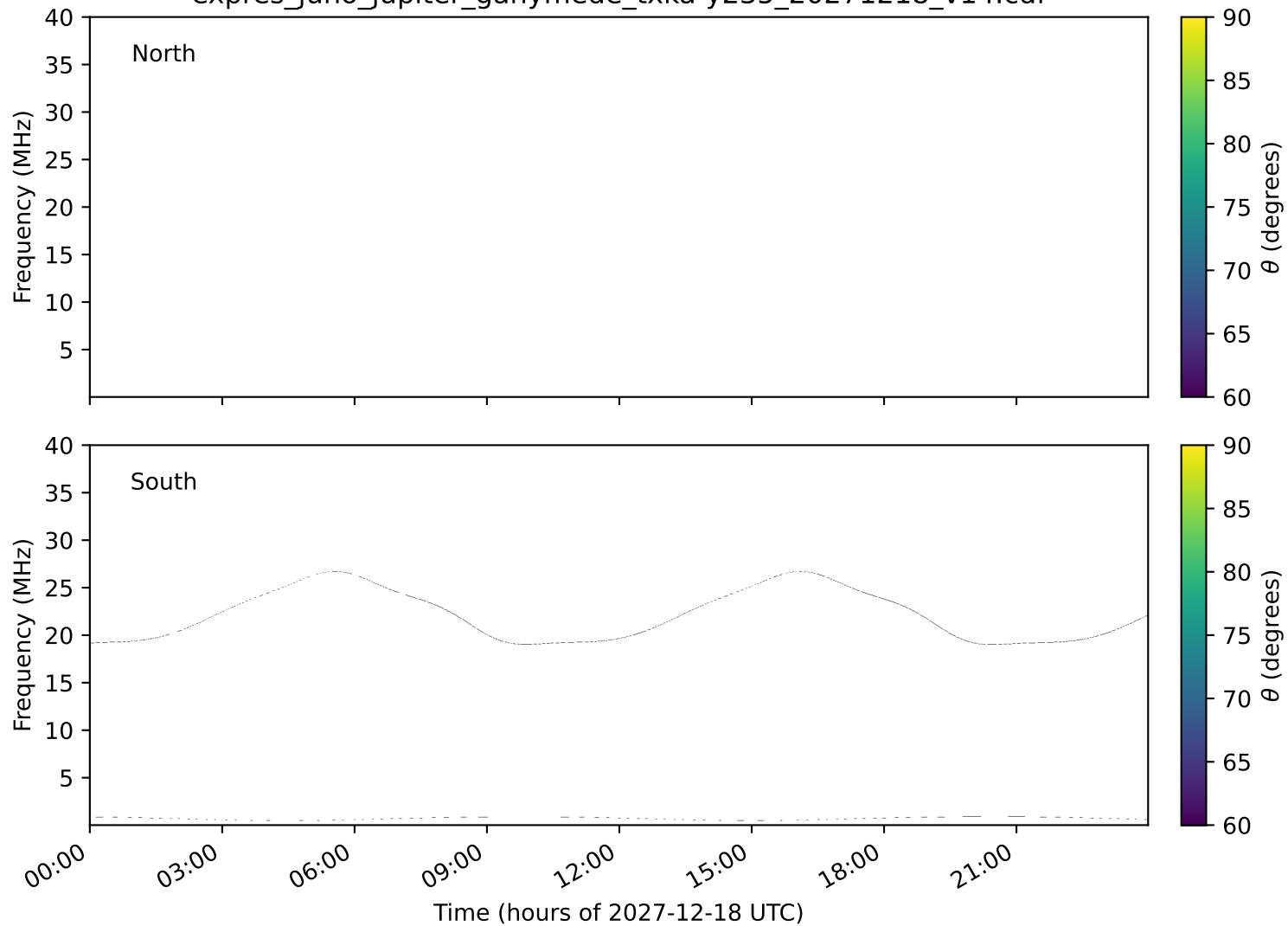
expres_juno_jupiter_ganymede_txka-y235_20271218_v14.cdf
