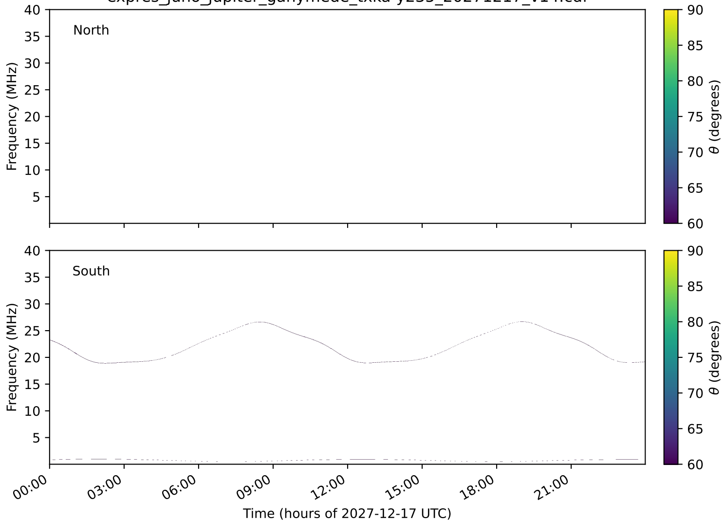
expres_juno_jupiter_ganymede_txka-y235_20271217_v14.cdf
