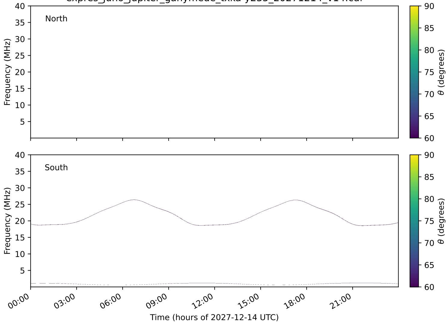
expres_juno_jupiter_ganymede_txka-y235_20271214_v14.cdf
