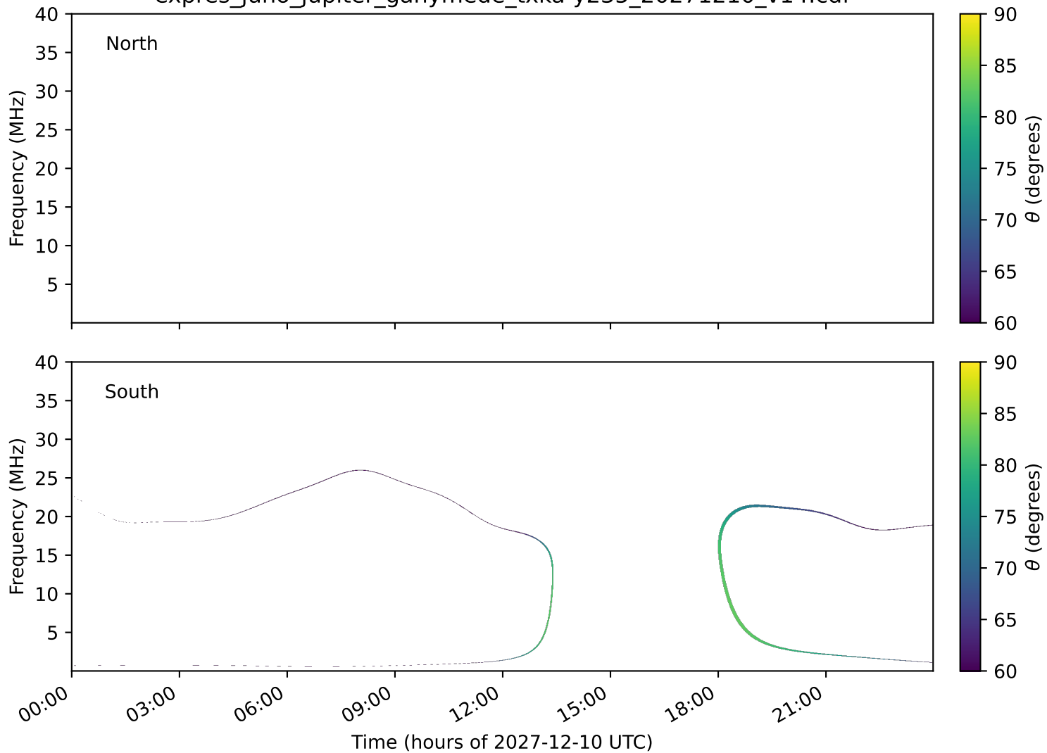
expres_juno_jupiter_ganymede_txka-y235_20271210_v14.cdf
