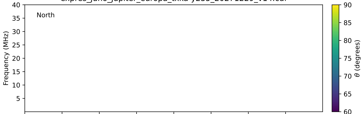
expres_juno_jupiter_europa_txka-y235_20271229_v14.cdf
