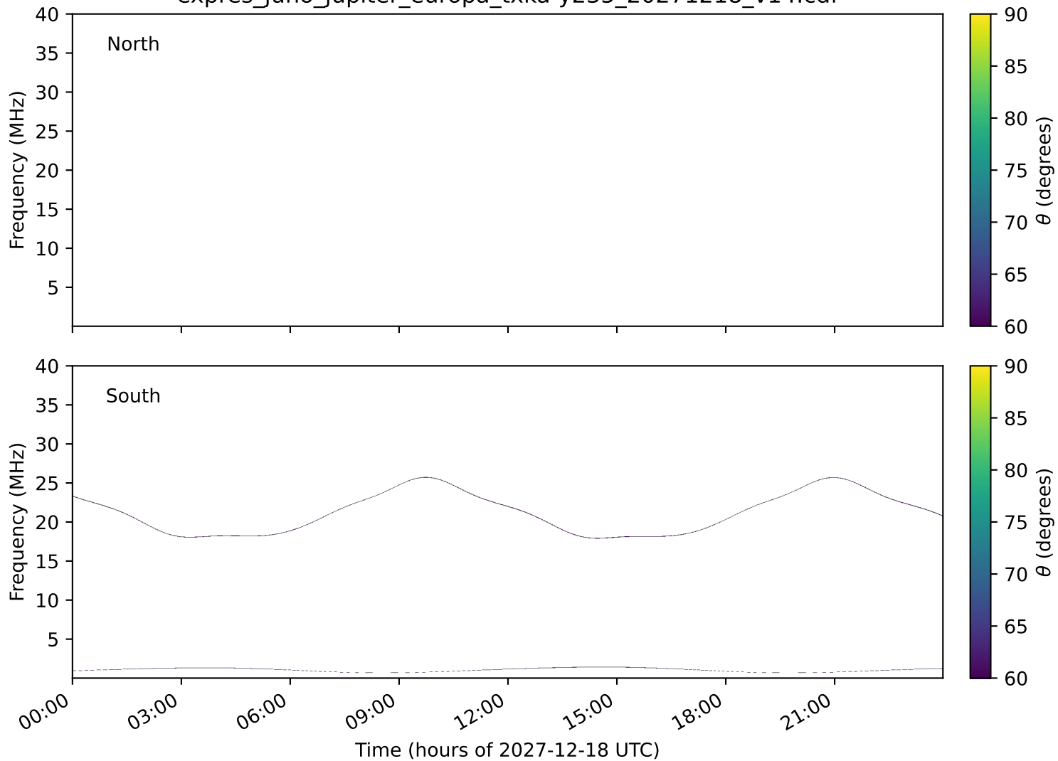
expres_juno_jupiter_europa_txka-y235_20271218_v14.cdf
