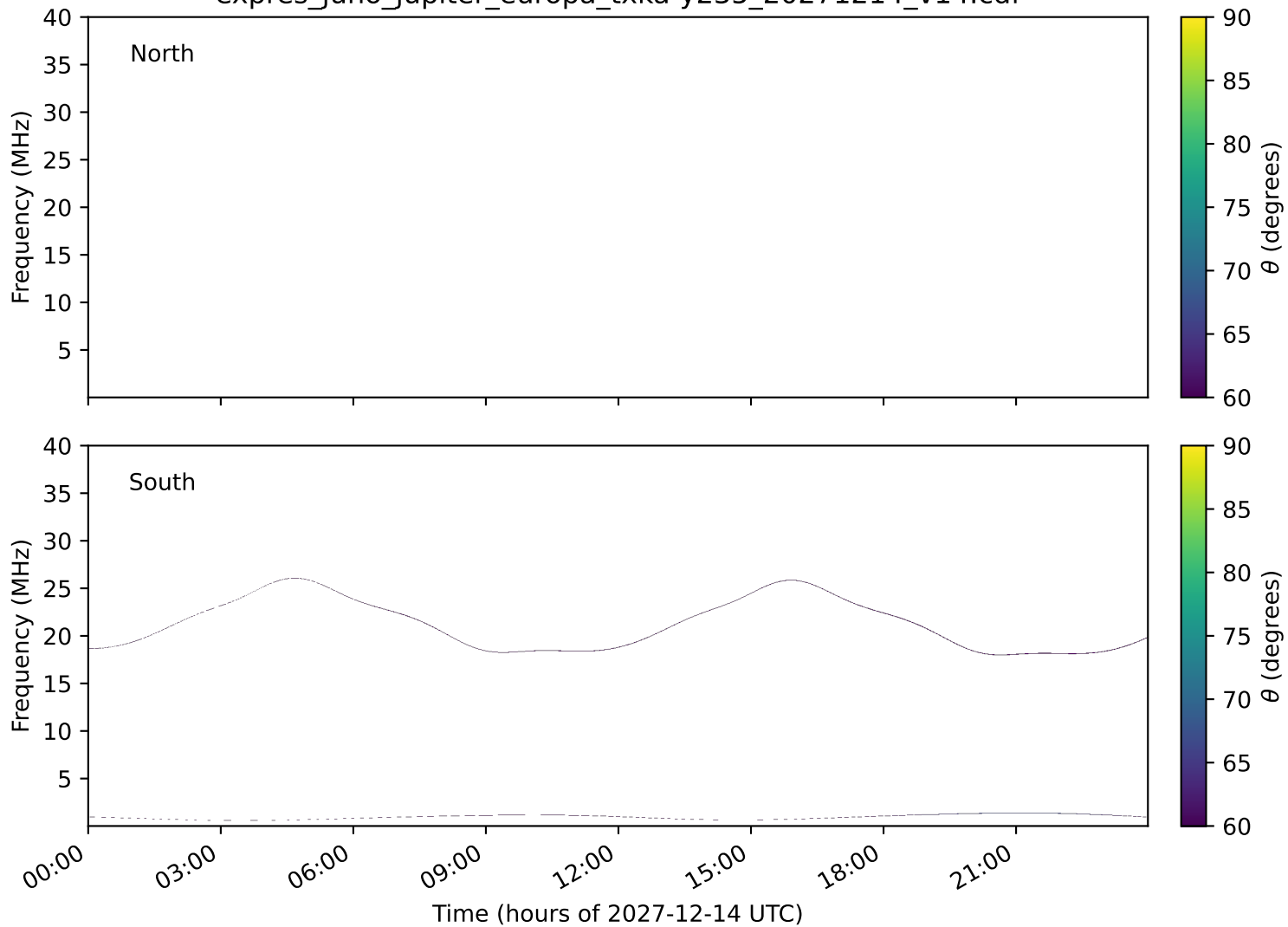
expres_juno_jupiter_europa_txka-y235_20271214_v14.cdf
