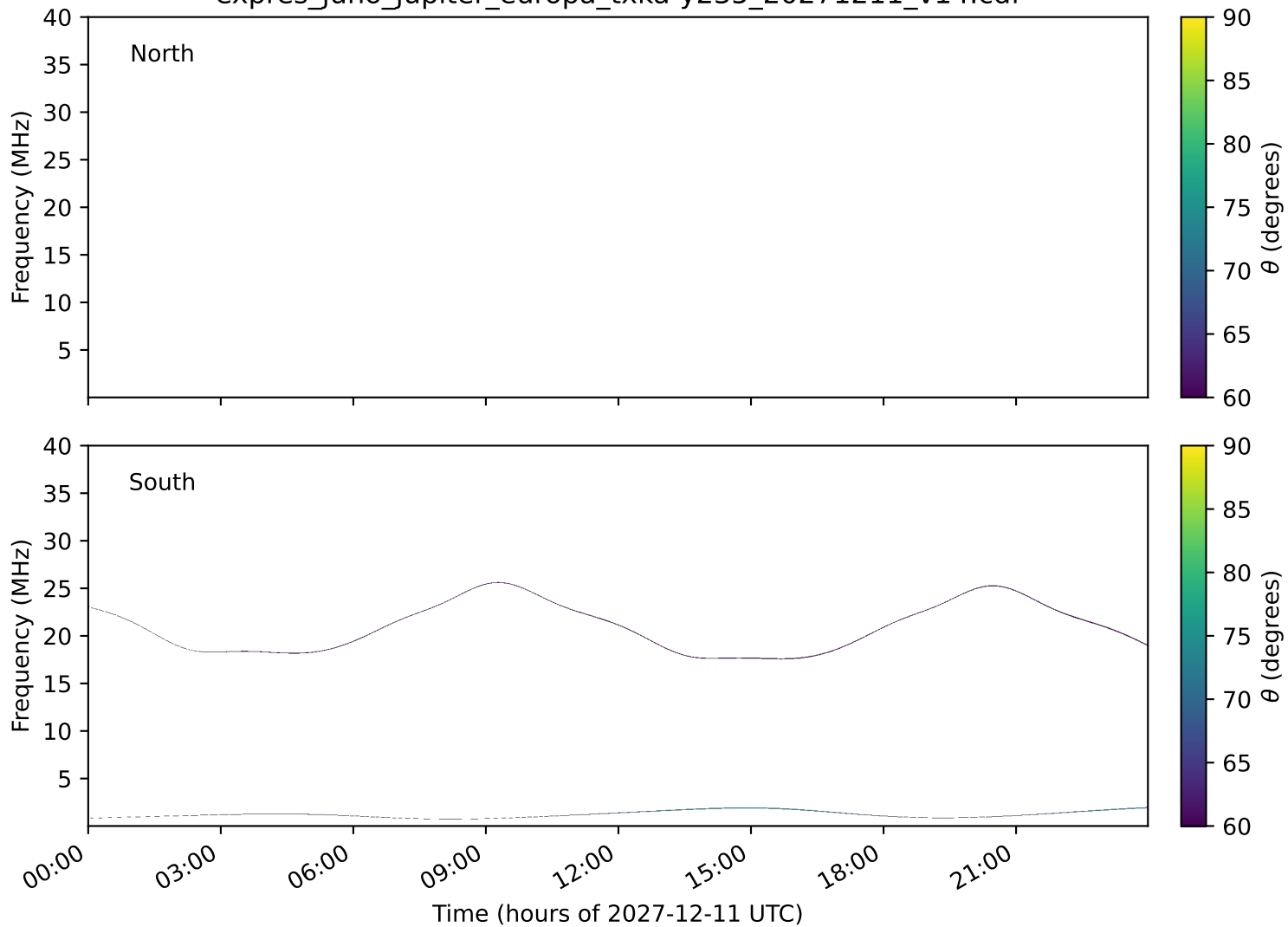
expres_juno_jupiter_europa_txka-y235_20271211_v14.cdf
