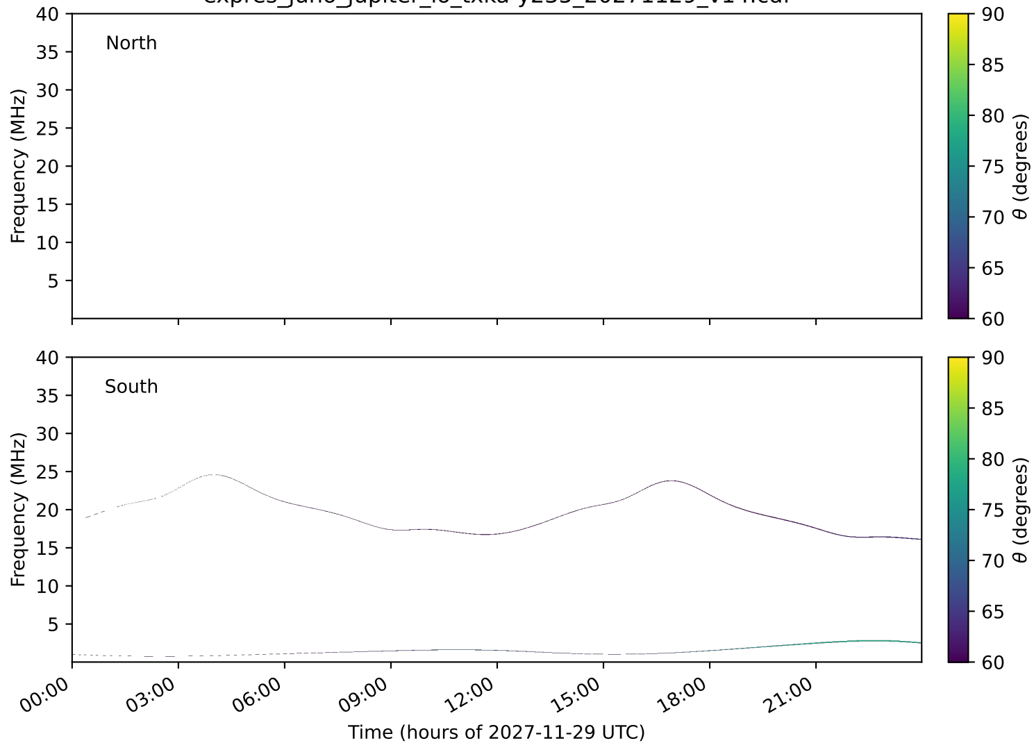
expres_juno_jupiter_io_txka-y235_20271129_v14.cdf
