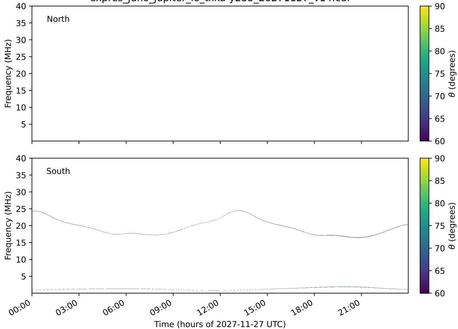
expres_juno_jupiter_io_txka-y235_20271127_v14.cdf
