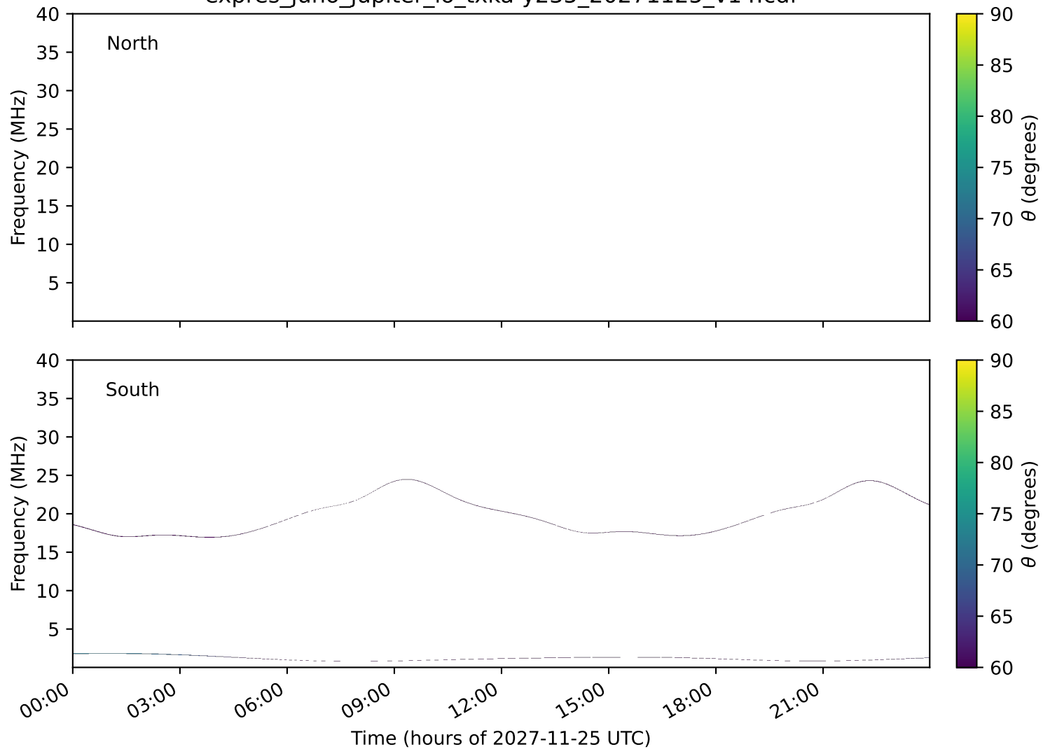
expres_juno_jupiter_io_txka-y235_20271125_v14.cdf
