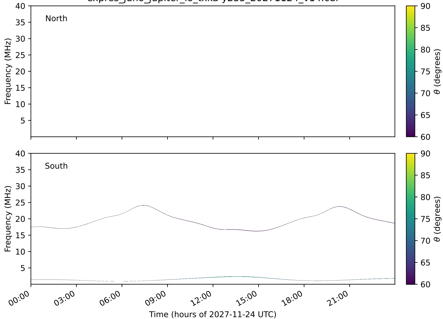
expres_juno_jupiter_io_txka-y235_20271124_v14.cdf
