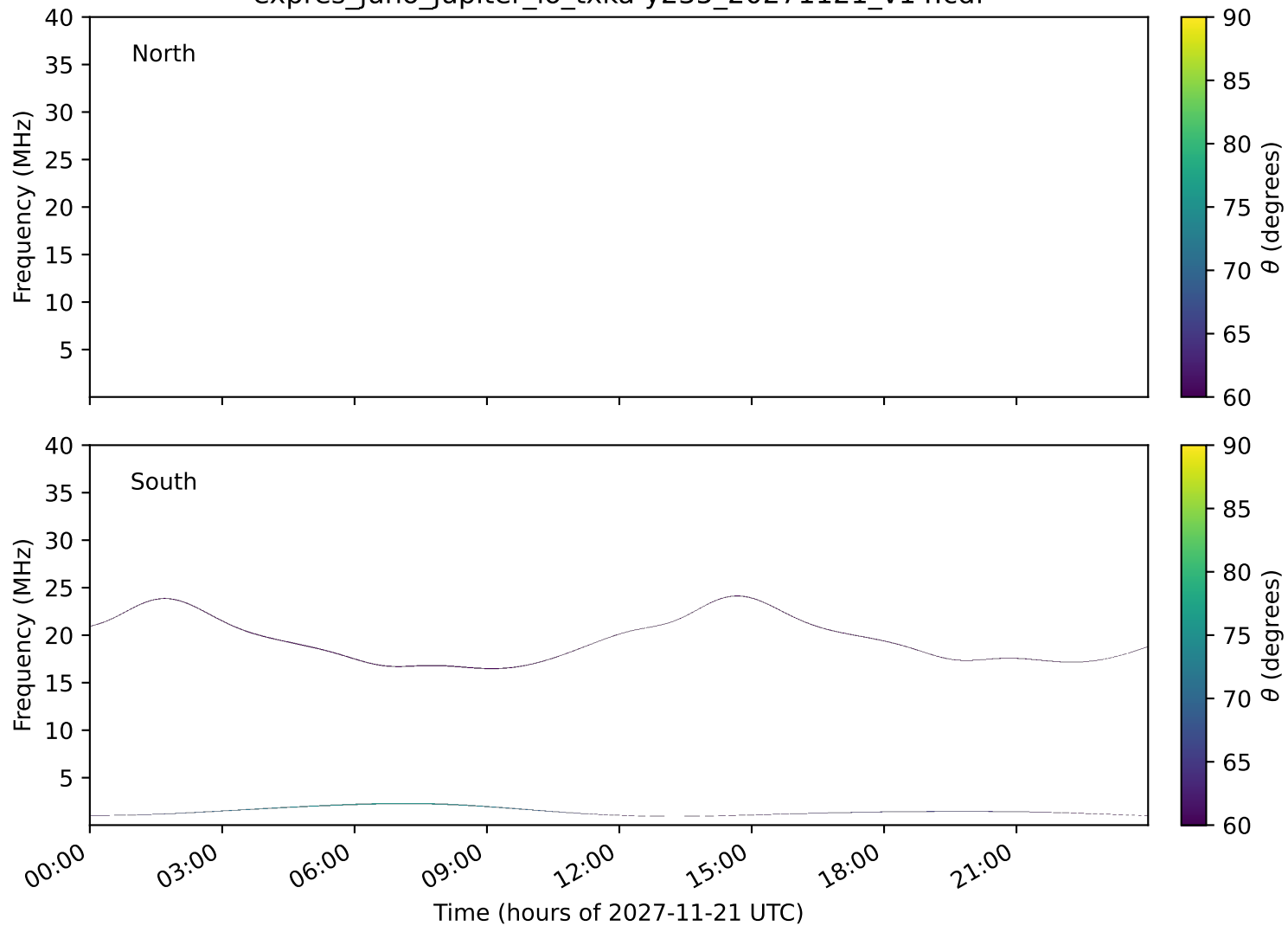
expres_juno_jupiter_io_txka-y235_20271121_v14.cdf
