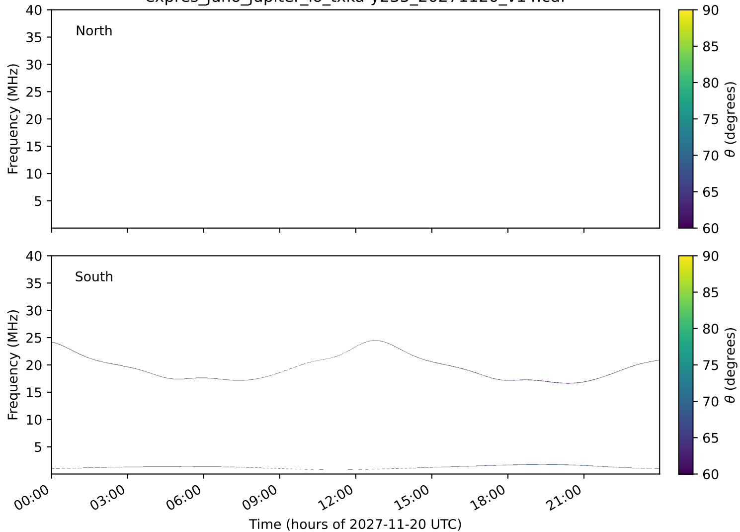
expres_juno_jupiter_io_txka-y235_20271120_v14.cdf
