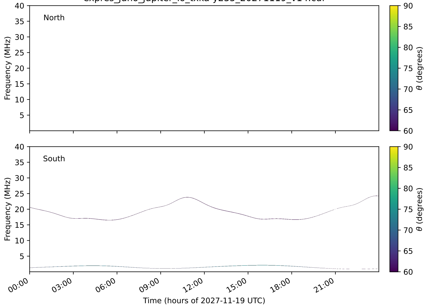
expres_juno_jupiter_io_txka-y235_20271119_v14.cdf
