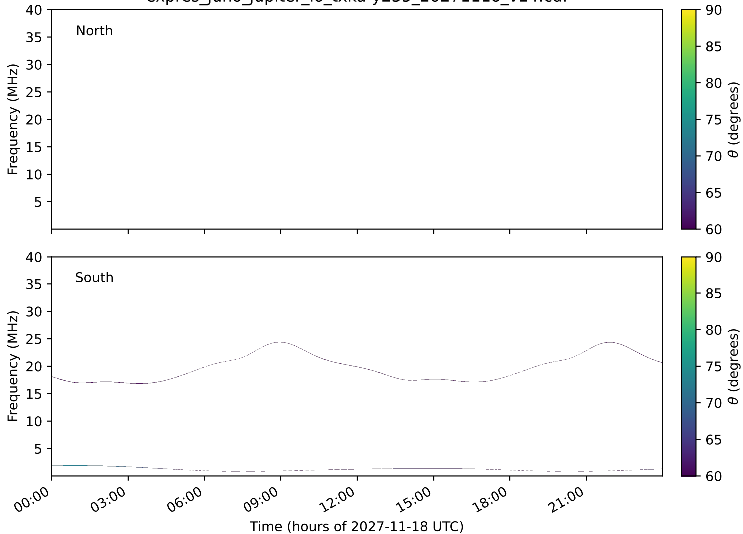
expres_juno_jupiter_io_txka-y235_20271118_v14.cdf
