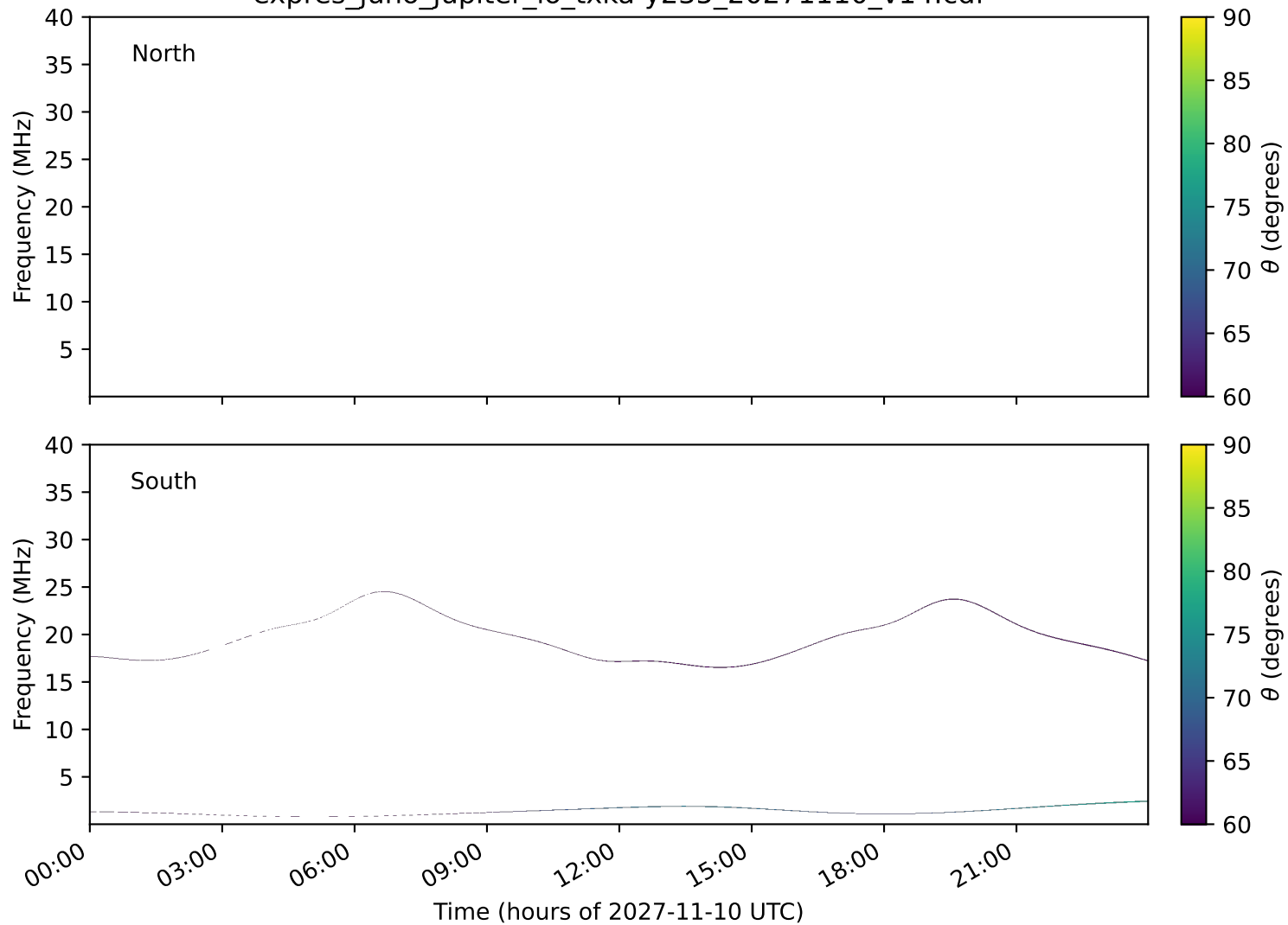
expres_juno_jupiter_io_txka-y235_20271110_v14.cdf
