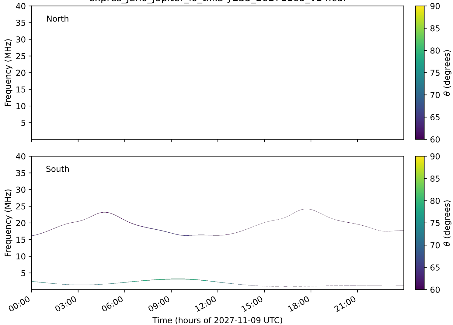
expres_juno_jupiter_io_txka-y235_20271109_v14.cdf
