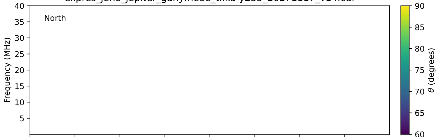
expres_juno_jupiter_ganymede_txka-y235_20271117_v14.cdf
