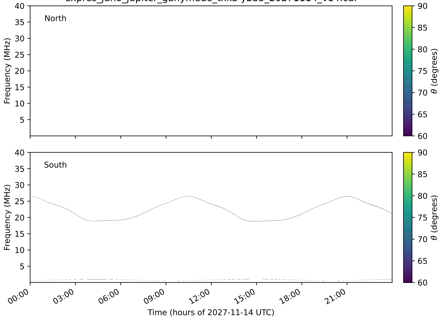
expres_juno_jupiter_ganymede_txka-y235_20271114_v14.cdf
