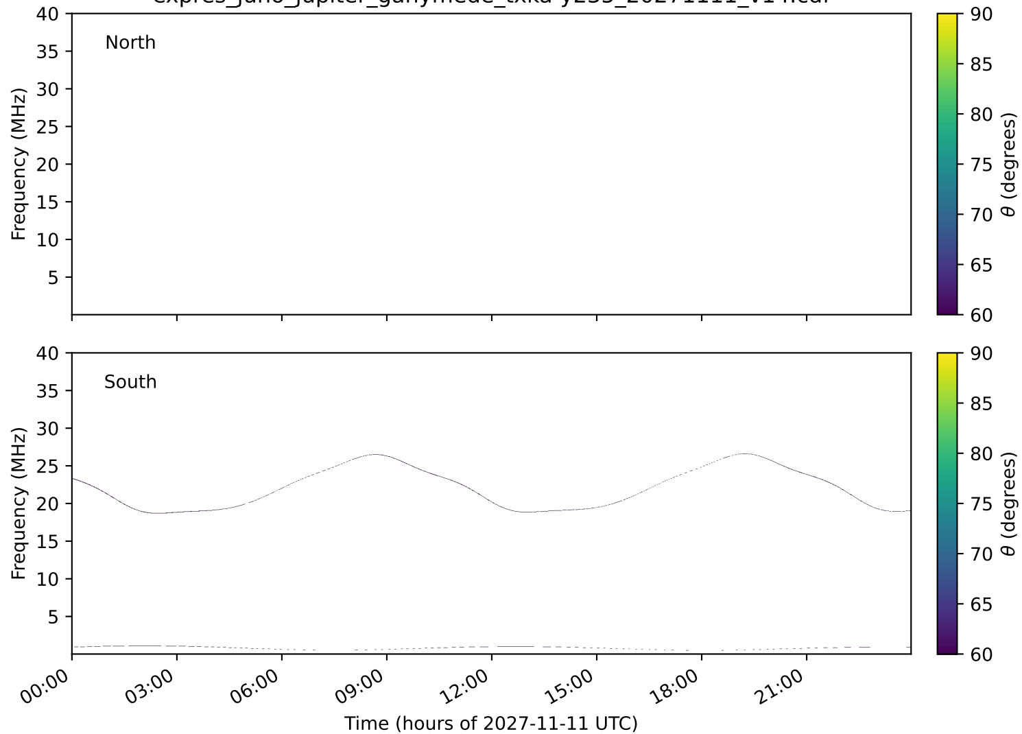
expres_juno_jupiter_ganymede_txka-y235_20271111_v14.cdf
