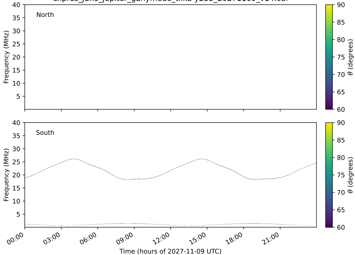
expres_juno_jupiter_ganymede_txka-y235_20271109_v14.cdf
