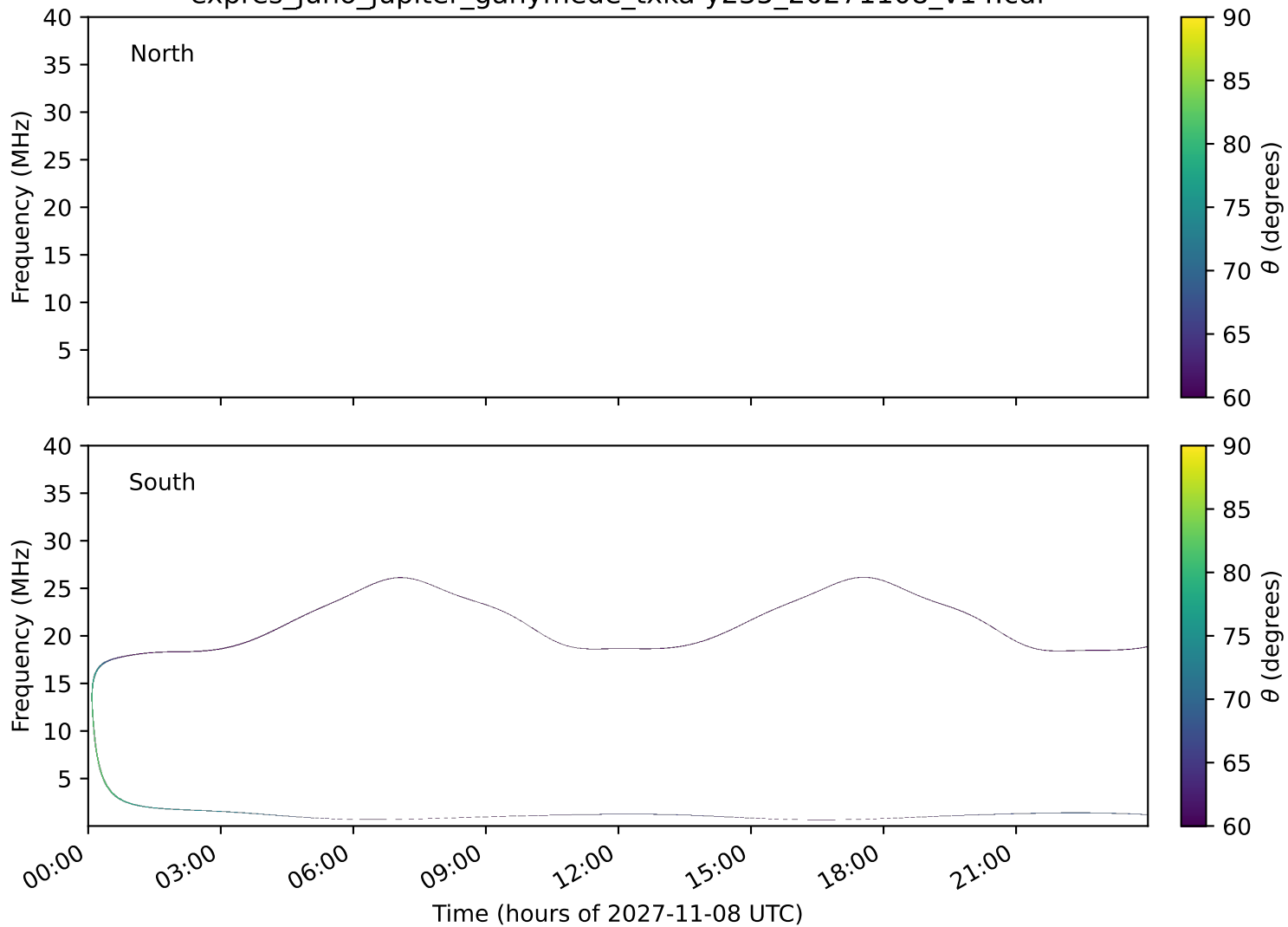
expres_juno_jupiter_ganymede_txka-y235_20271108_v14.cdf
