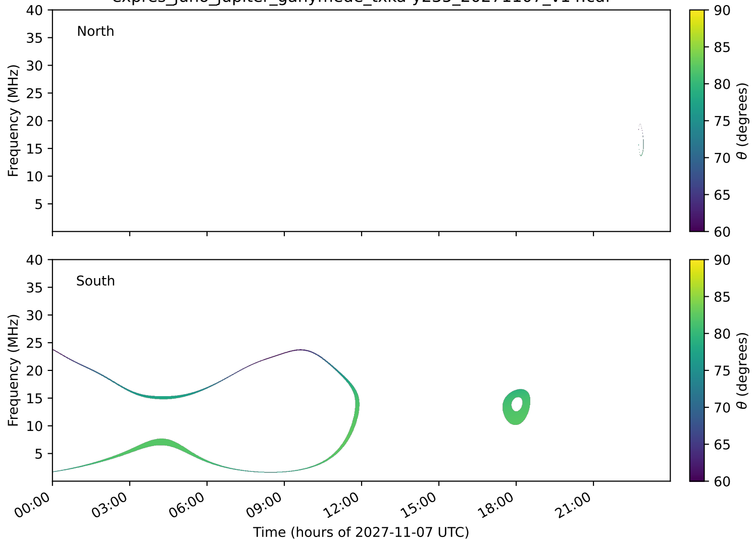
expres_juno_jupiter_ganymede_txka-y235_20271107_v14.cdf
