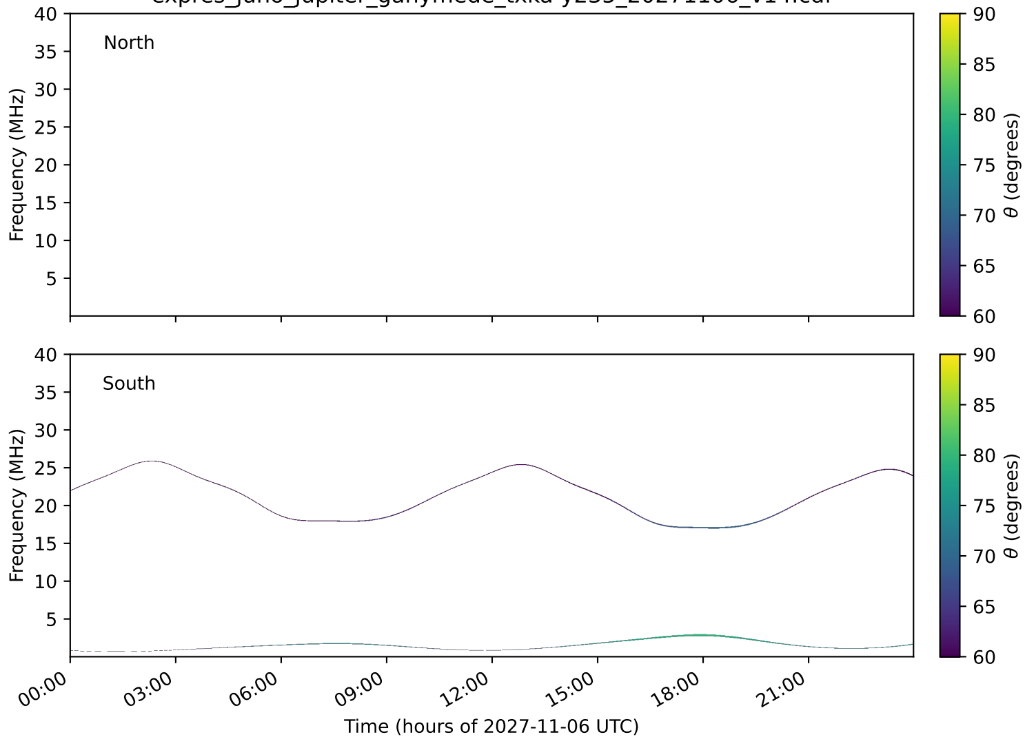
expres_juno_jupiter_ganymede_txka-y235_20271106_v14.cdf
