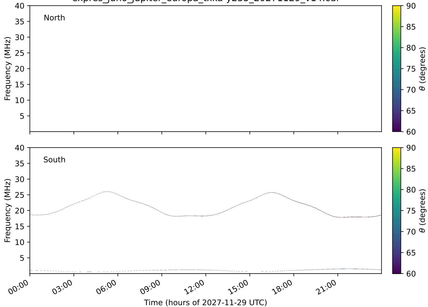
expres_juno_jupiter_europa_txka-y235_20271129_v14.cdf
