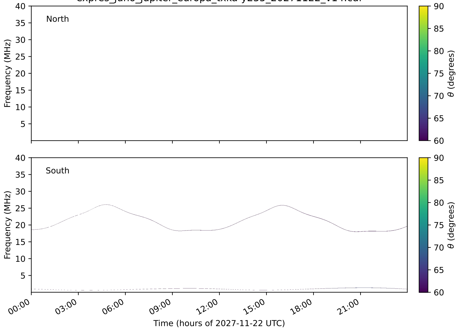
expres_juno_jupiter_europa_txka-y235_20271122_v14.cdf
