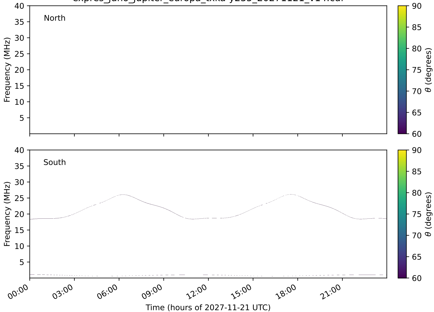
expres_juno_jupiter_europa_txka-y235_20271121_v14.cdf
