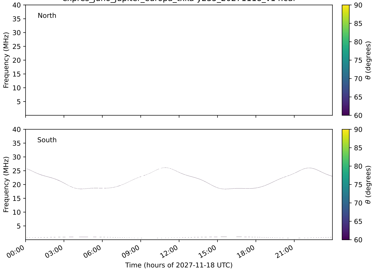
expres_juno_jupiter_europa_txka-y235_20271118_v14.cdf
