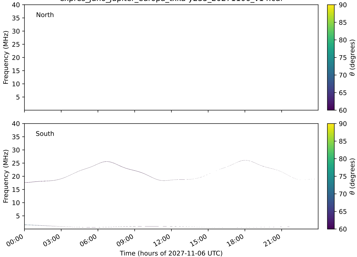
expres_juno_jupiter_europa_txka-y235_20271106_v14.cdf
