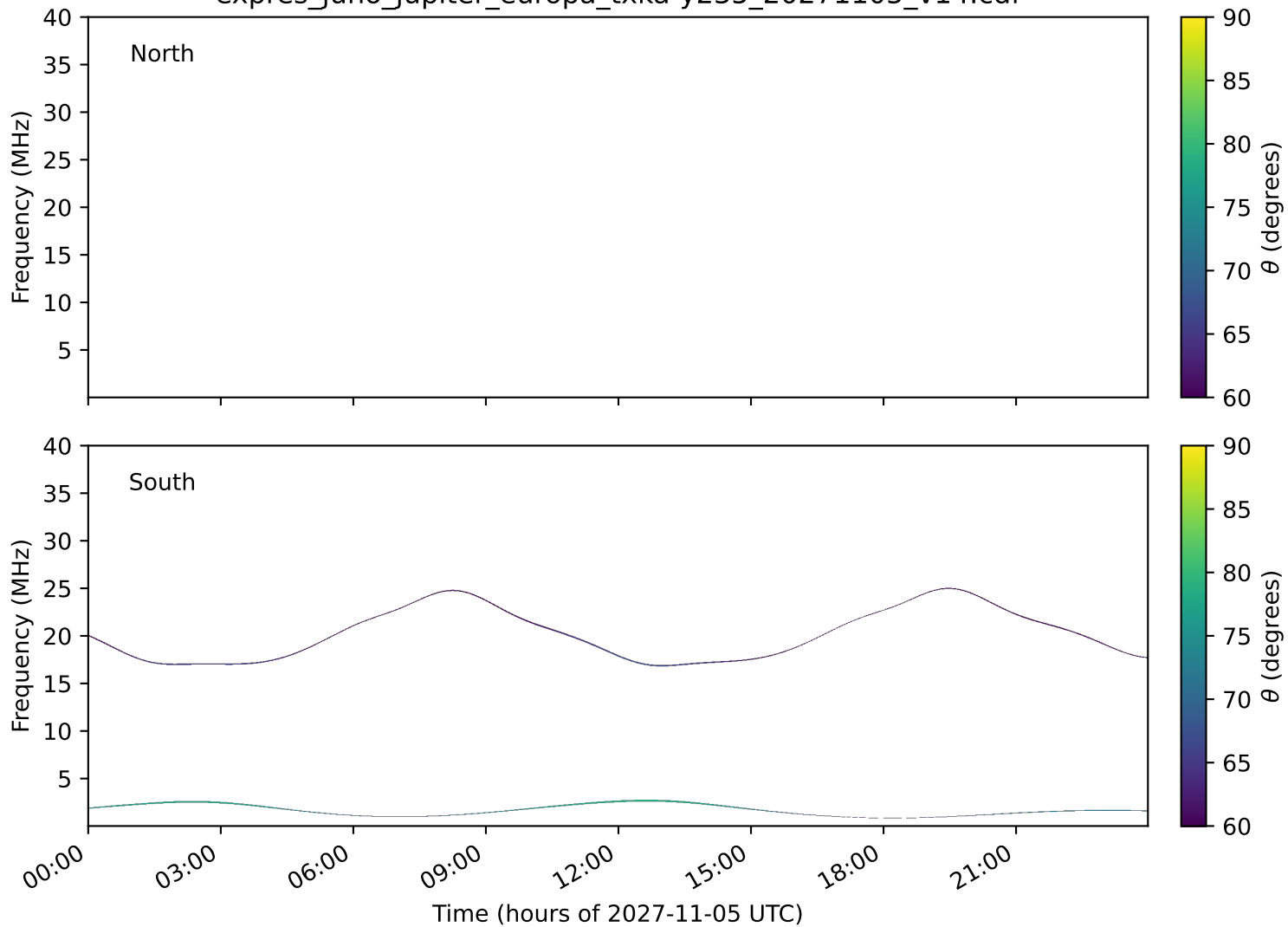
expres_juno_jupiter_europa_txka-y235_20271105_v14.cdf
