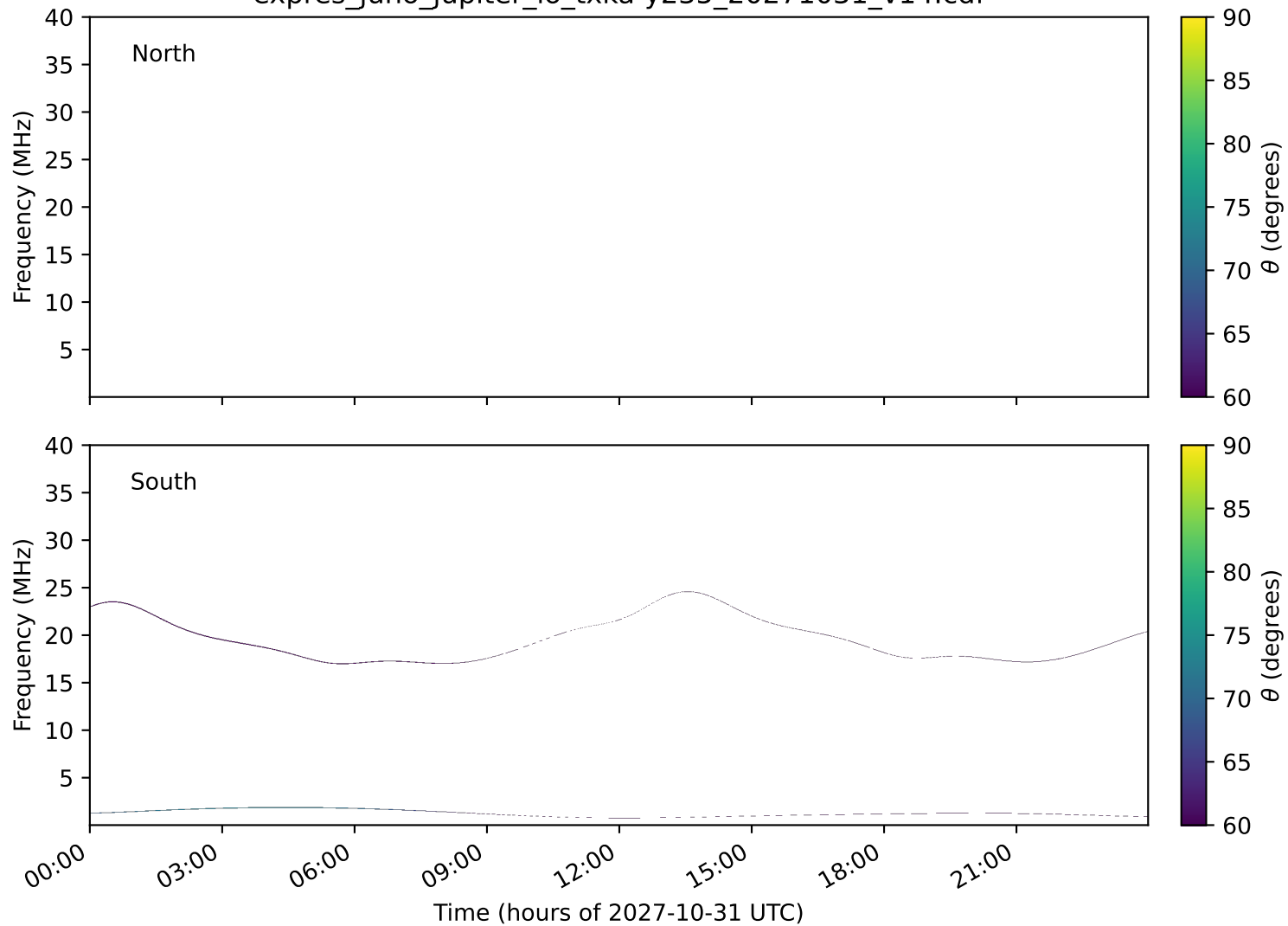
expres_juno_jupiter_io_txka-y235_20271031_v14.cdf
