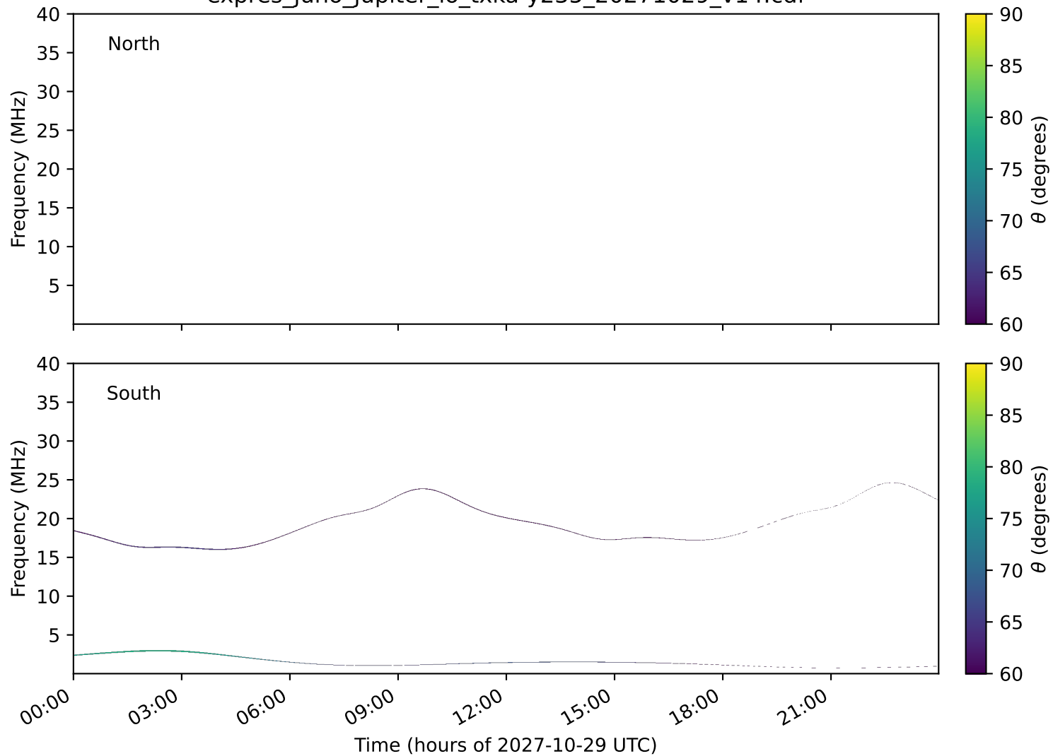
expres_juno_jupiter_io_txka-y235_20271029_v14.cdf
