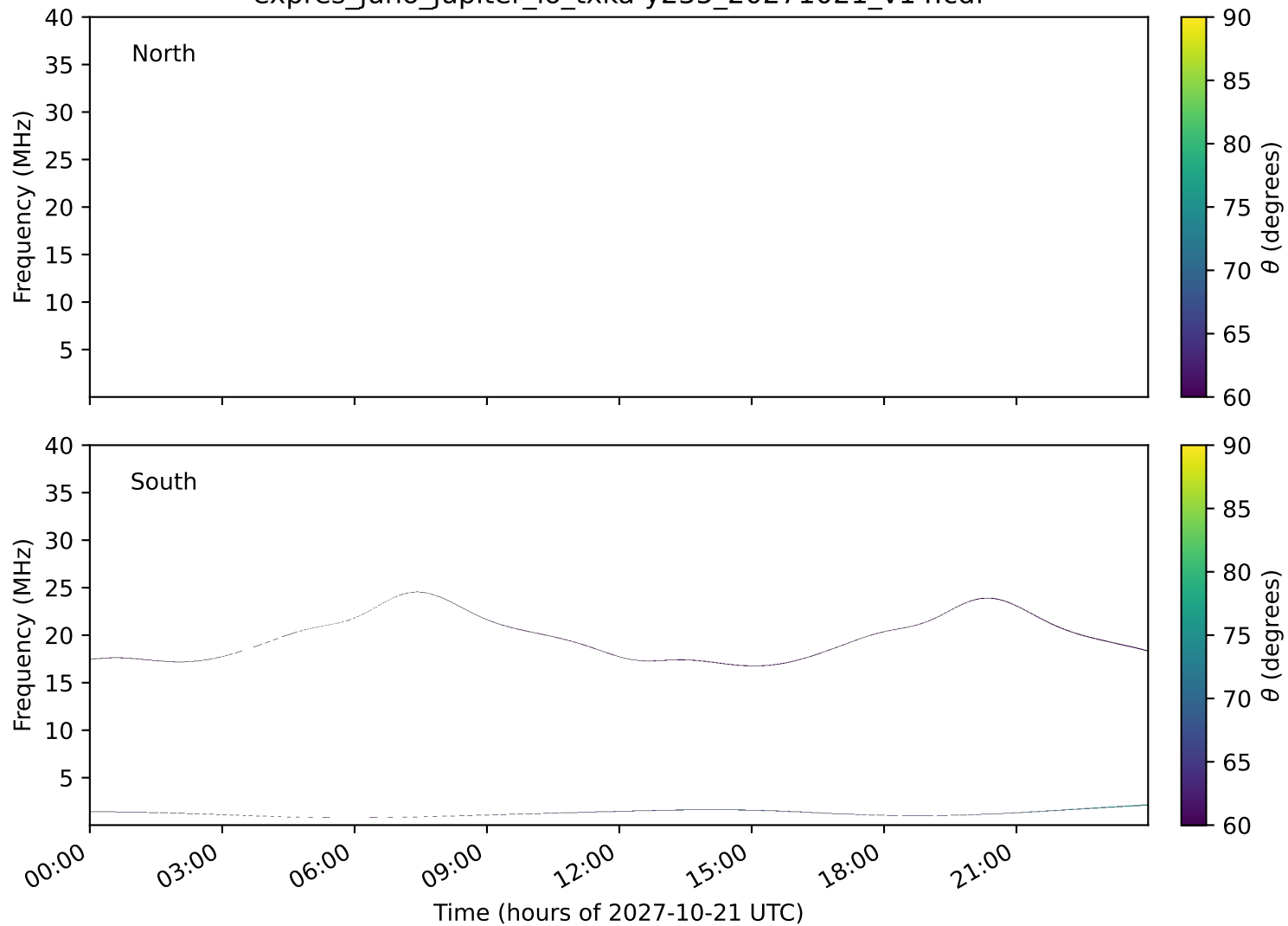
expres_juno_jupiter_io_txka-y235_20271021_v14.cdf
