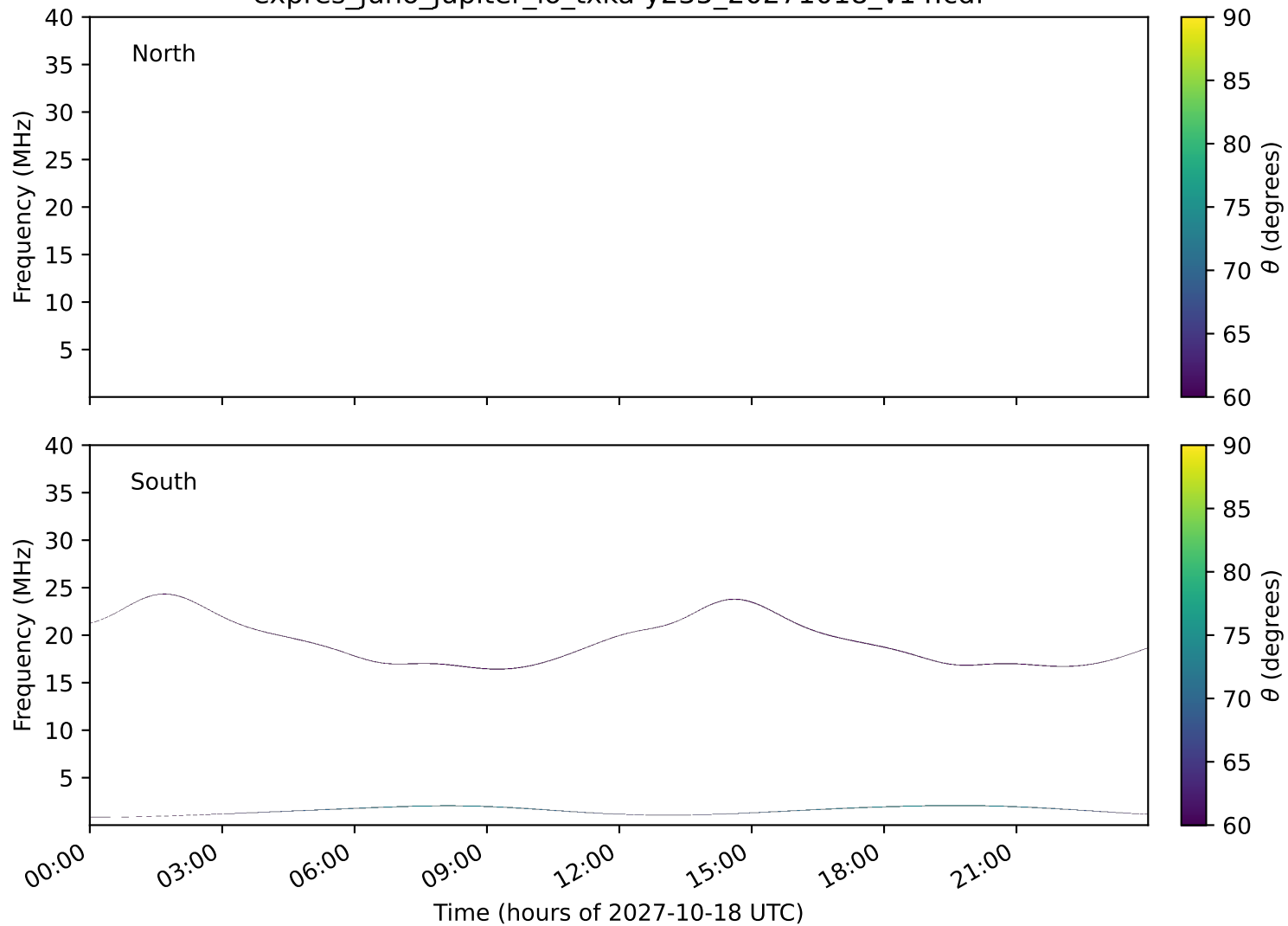
expres_juno_jupiter_io_txka-y235_20271018_v14.cdf
