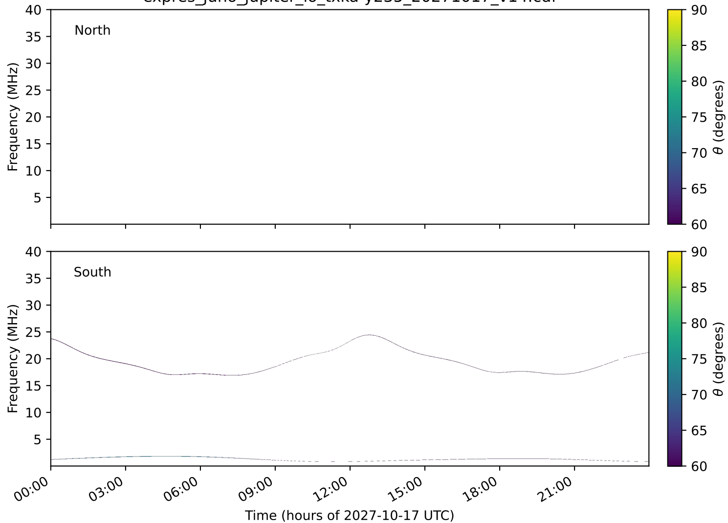
expres_juno_jupiter_io_txka-y235_20271017_v14.cdf
