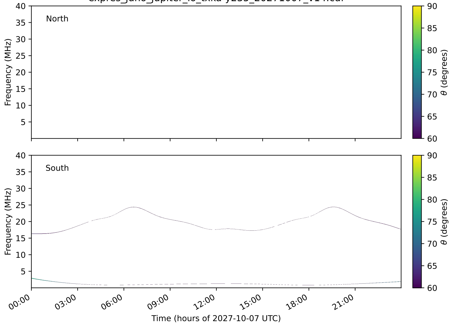
expres_juno_jupiter_io_txka-y235_20271007_v14.cdf
