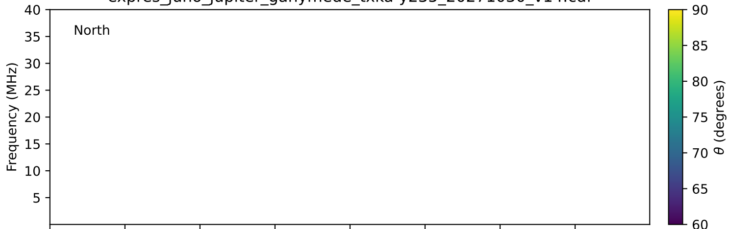
expres_juno_jupiter_ganymede_txka-y235_20271030_v14.cdf
