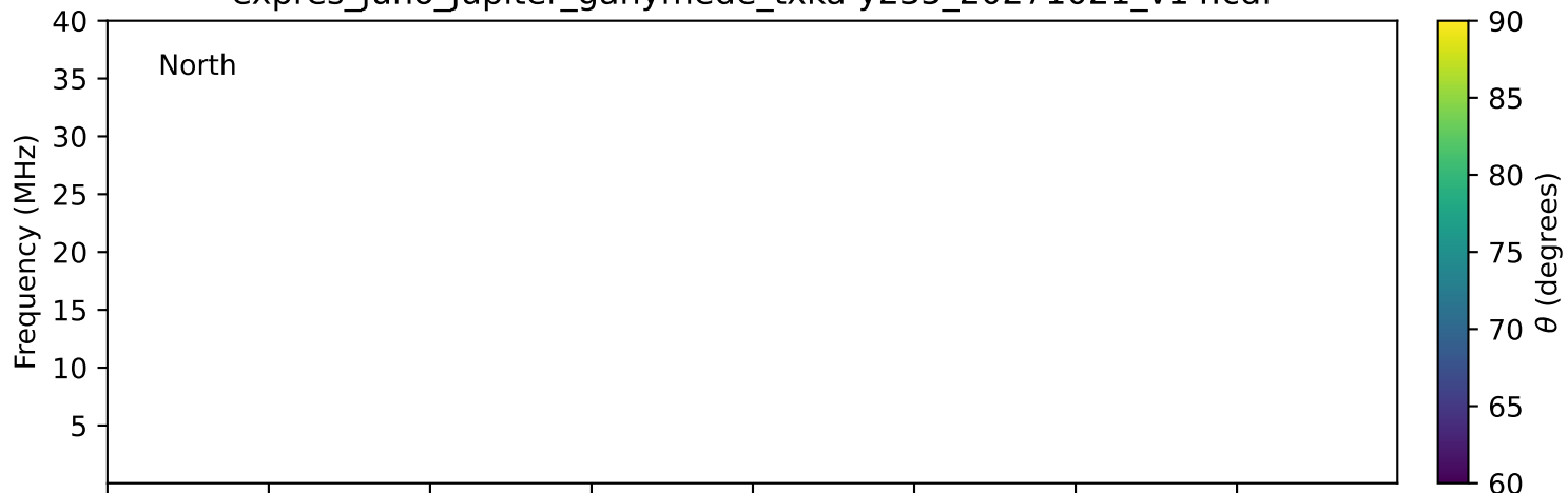
expres_juno_jupiter_ganymede_txka-y235_20271021_v14.cdf
