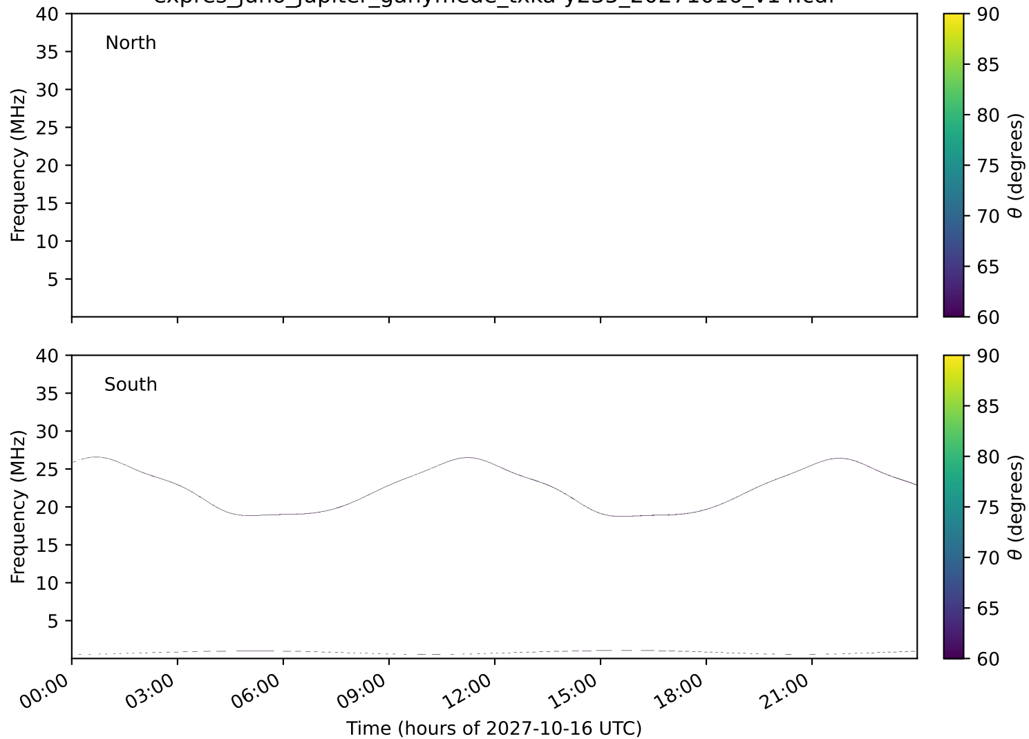
expres_juno_jupiter_ganymede_txka-y235_20271016_v14.cdf
