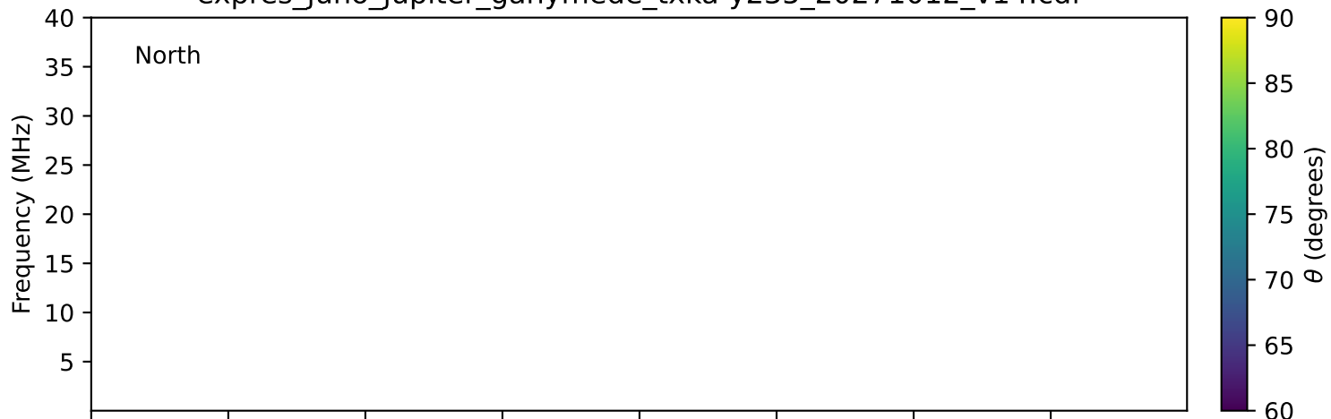
expres_juno_jupiter_ganymede_txka-y235_20271012_v14.cdf
