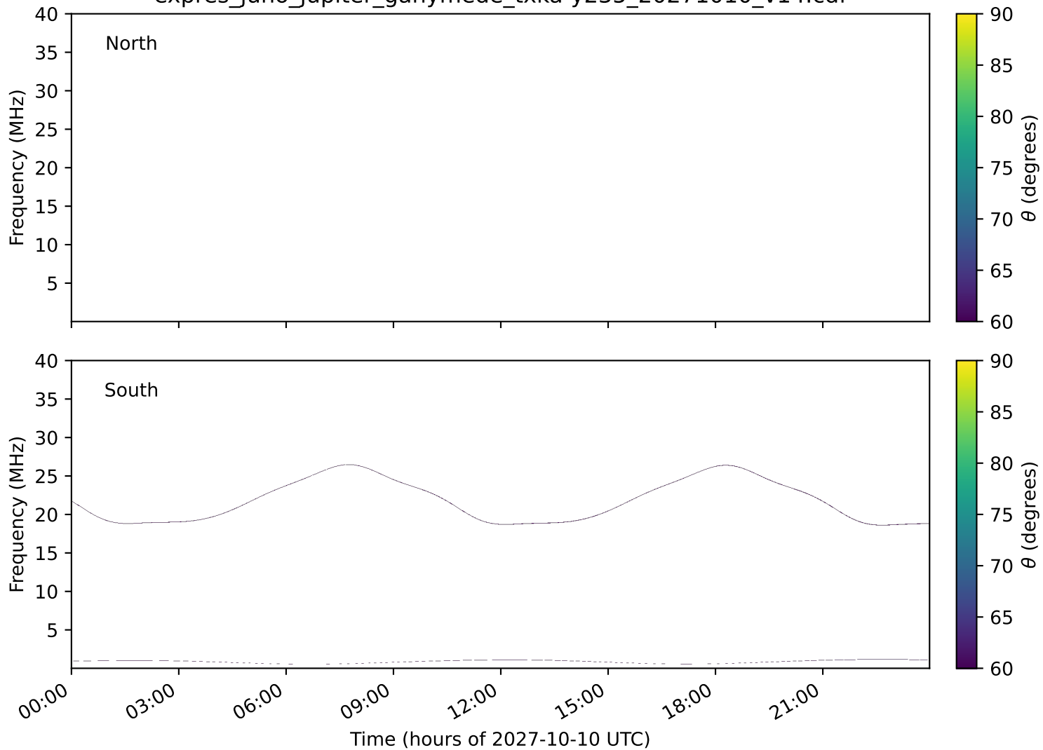
expres_juno_jupiter_ganymede_txka-y235_20271010_v14.cdf
