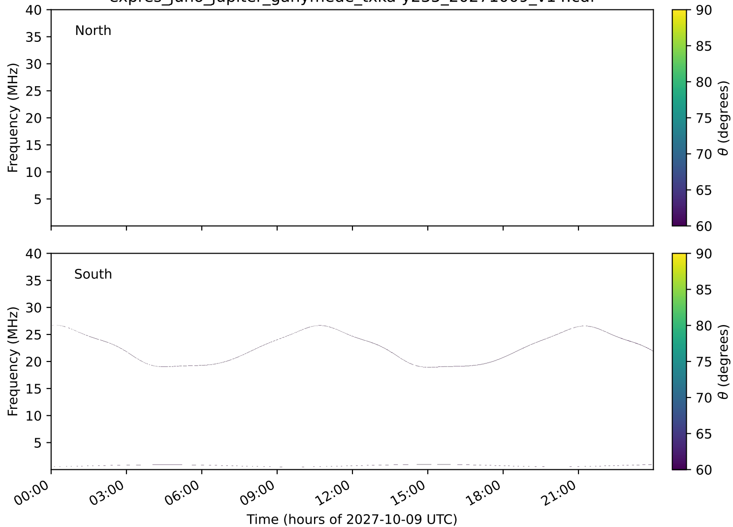
expres_juno_jupiter_ganymede_txka-y235_20271009_v14.cdf
