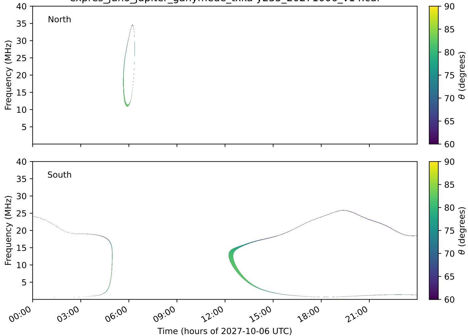
expres_juno_jupiter_ganymede_txka-y235_20271006_v14.cdf
