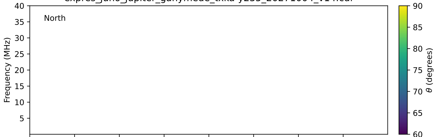
expres_juno_jupiter_ganymede_txka-y235_20271004_v14.cdf
