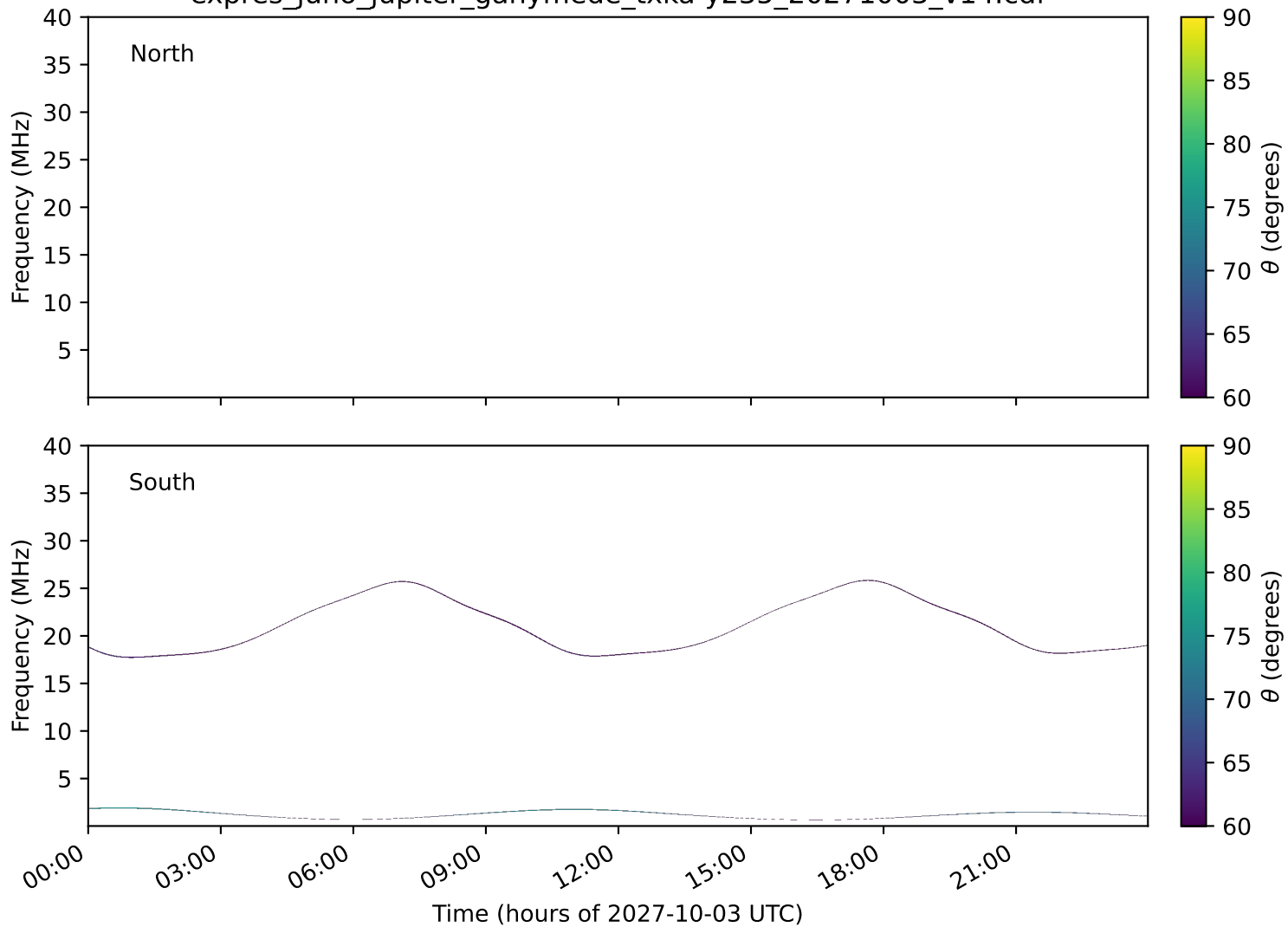
expres_juno_jupiter_ganymede_txka-y235_20271003_v14.cdf
