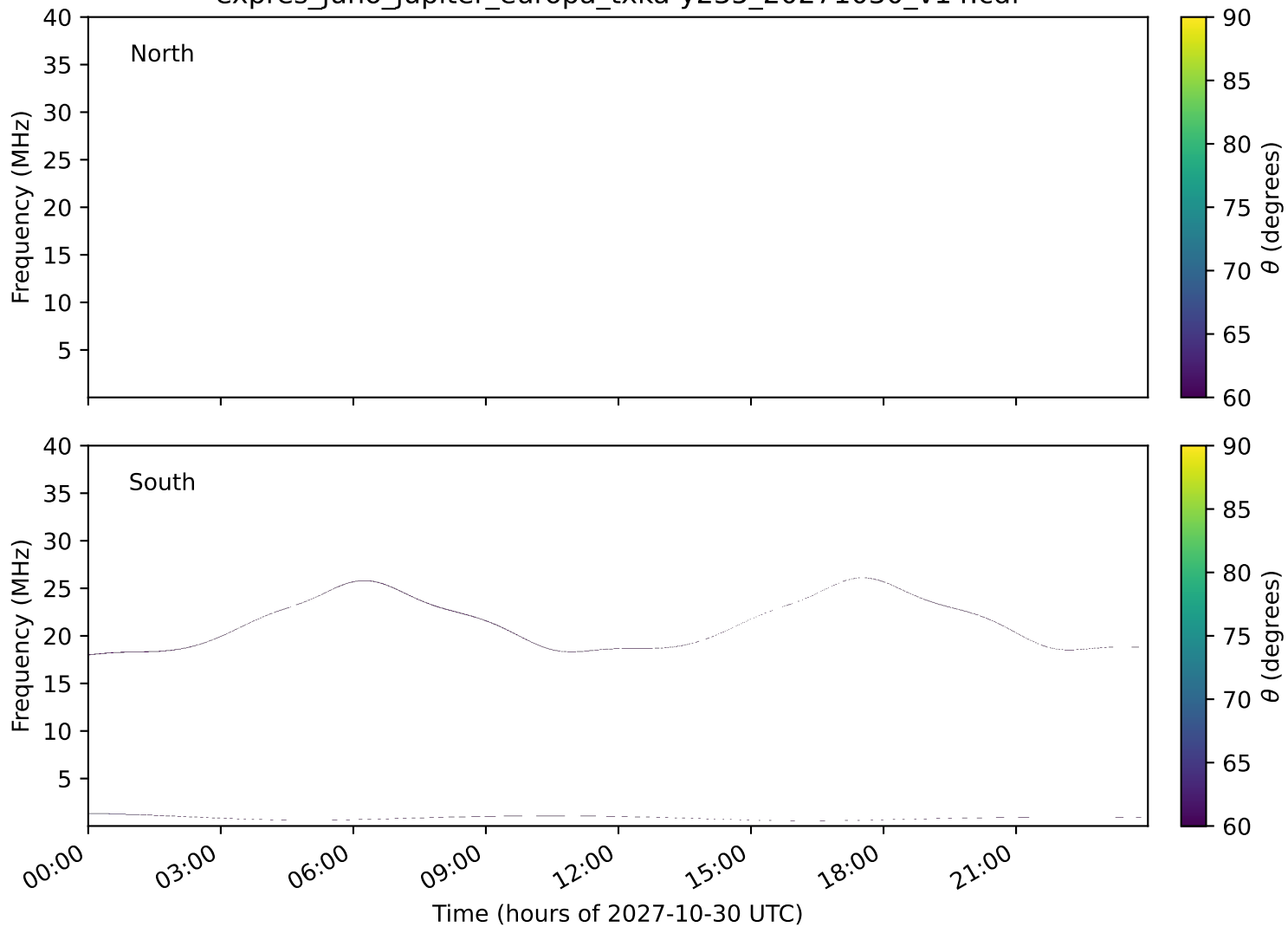
expres_juno_jupiter_europa_txka-y235_20271030_v14.cdf
