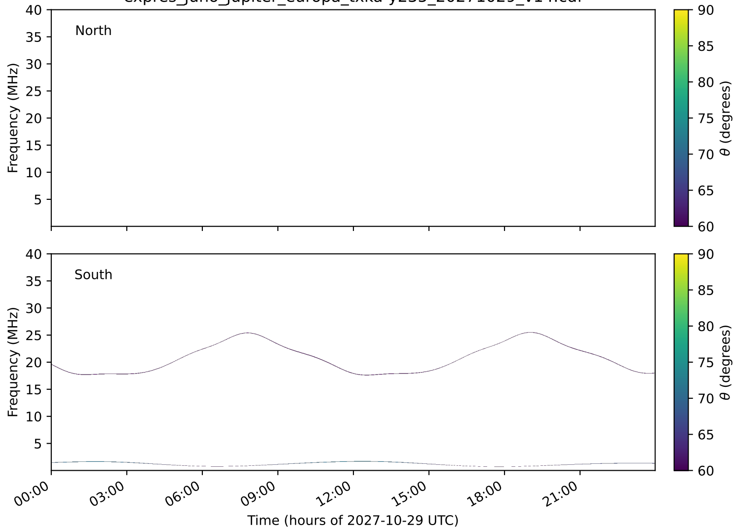
expres_juno_jupiter_europa_txka-y235_20271029_v14.cdf
