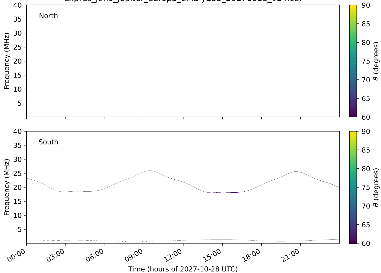
expres_juno_jupiter_europa_txka-y235_20271028_v14.cdf
